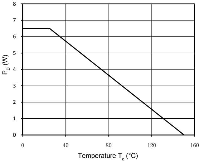
Figure 9. Power Dissipation
