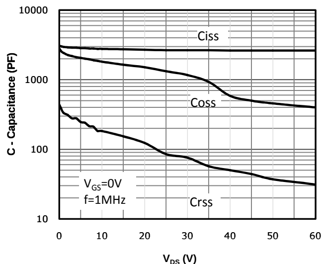
Fig 6: Capacitance Characteristics
