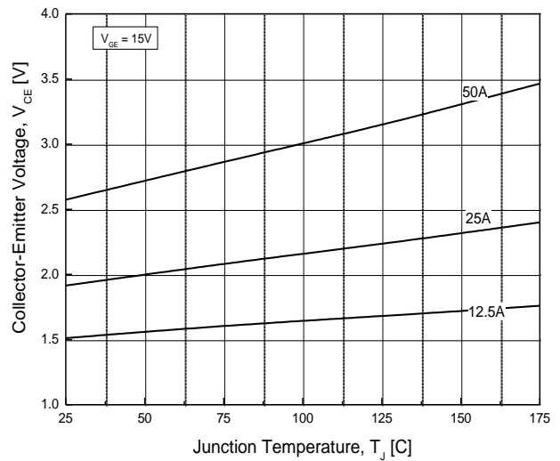
Fig.4 Typical Collector-Emittor Saturation Voltage -Junction Temperature
