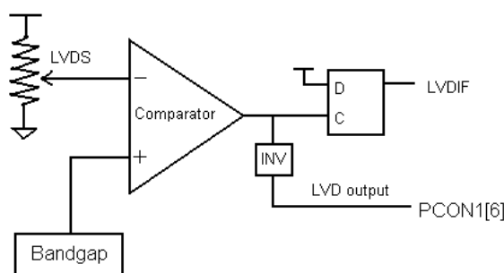
Figure 16 LVD block diagram
