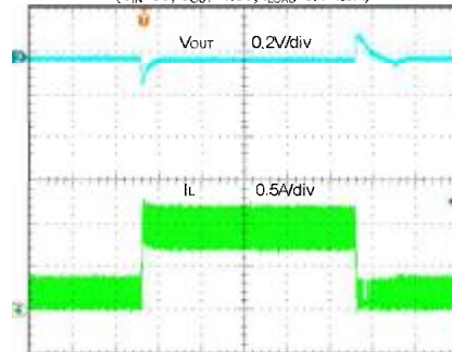
Load Transient
