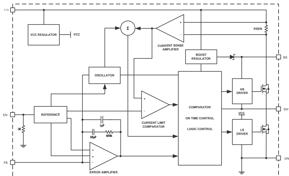
Figure 2. HM8112 Block Diagram
